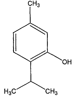
Timol C 10 H 14 O
