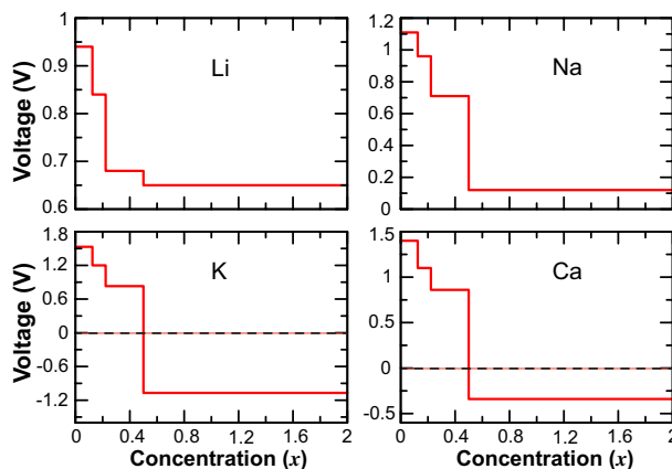
Fig. 8 (Color online) Calculated voltage profile as a function of concentration for double side adsorption.
