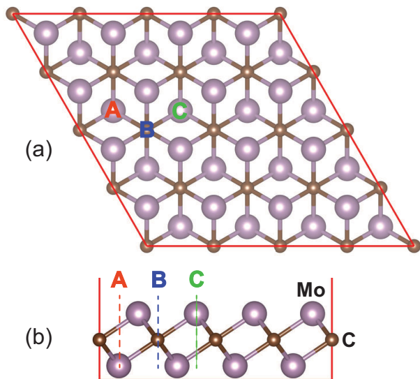
Fig. 1 (Color online) Top and side view of optimized structure of the \text{Mo}_2\text{C} monolayer. A, B and C represent the possible adsorption sites for metal atoms.
