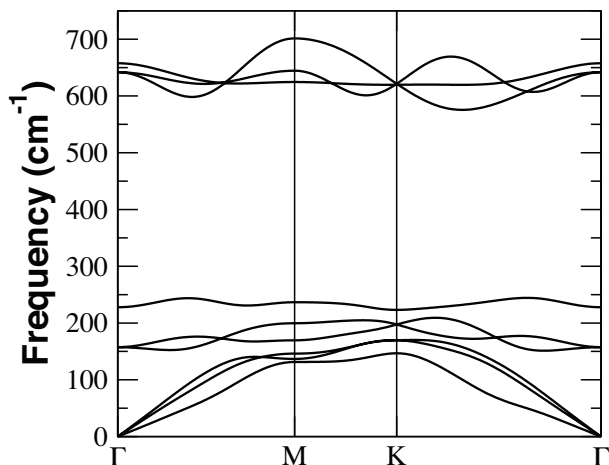
Fig. 2 (Color online) Calculated phonon dispersion along the high symmetry directions for the pristine \text{Mo}_2\text{C} monolayer.
