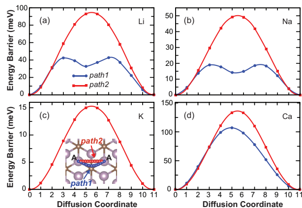
Fig. 5 (Color online) Diffusion barrier profiles of (a) Li, (b) Na, (c) K and (d) Ca. The inset of (c) depicts the two possible optimized migration pathways between two nearest A sites.
