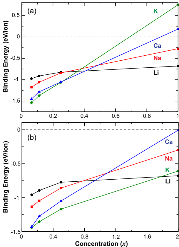
Fig. 7 (Color online) Binding energy as a function of metal atom concentration ( x ): (a) single side and (b) double side adsorption.
