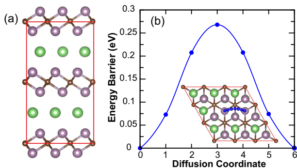
Fig. 6 (Color online) (a) Optimized structure of \text{Mo}_2\text{C-Li} complex and (b) diffusion barrier and path (see blue dots in the inset) of a Li ion.
