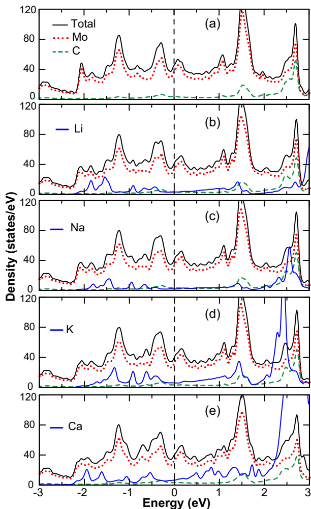
Fig. 4 (Color online) Total and partial DOS for (a) pristine, (b) Li, (c) Na, (d) K and (e) Ca doped Mo 2 C. The PDOS of the metal ions (multiplied with 100 for Li, Na and K and 25 for Ca) and C (multiplied with 4) atoms is enlarged in order to make them visible. The Fermi level is set to zero energy.
