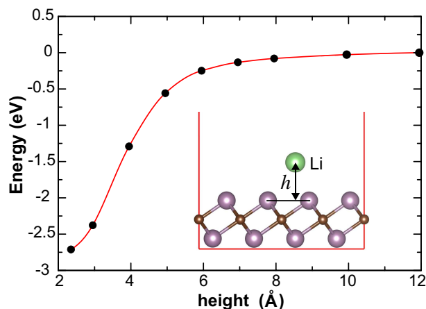
Fig. 3 (Color online) Change of total energy of Li- \text{Mo}_2\text{C} system as a function of vertical distance between the Li atom and the \text{Mo}_2\text{C} monolayer.
