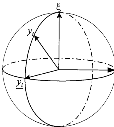
Figure 3. Lifting from S_{\frac{\pi}{2}}^2 configuration to S_{\alpha}^2 configuration.
