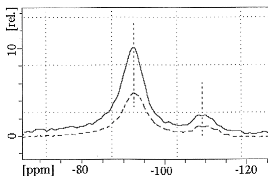
Figure 2. ^{29}\text{Si} MAS NMR spectra of 1,4-dioxane treated and untreated (dotted lines) bentonite samples
