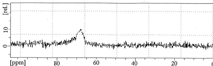
Figure 3. ^{13}\text{C} CP/MAS NMR spectrum of 1,4-dioxane treated bentonite sample
