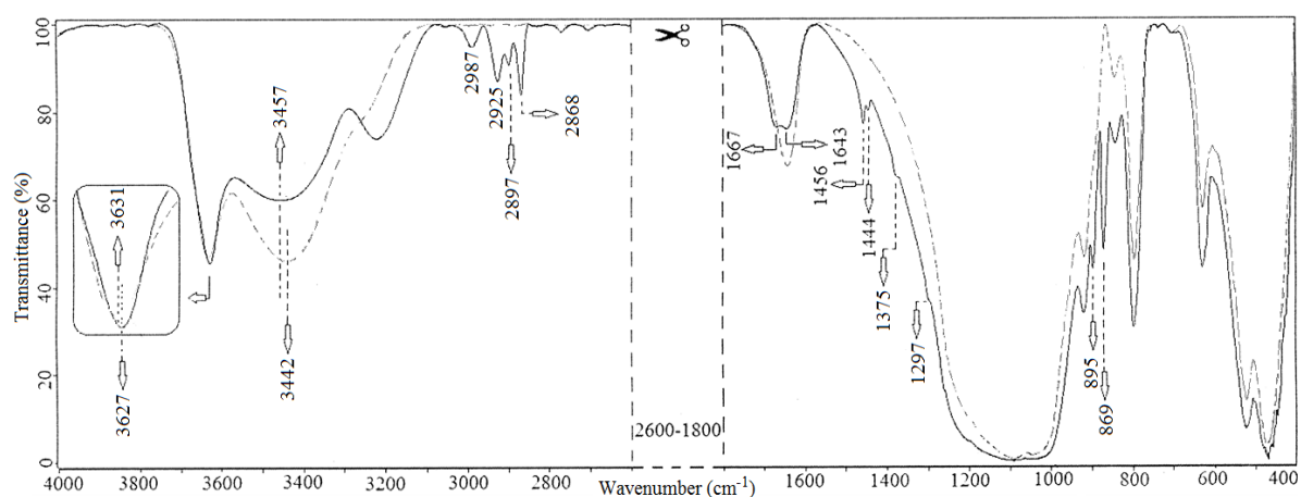
Figure 1. FT-IR spectra of 1,4-dioxane treated and untreated (dotted lines) bentonite samples
