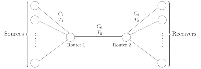
Fig. 2. Network topology.
