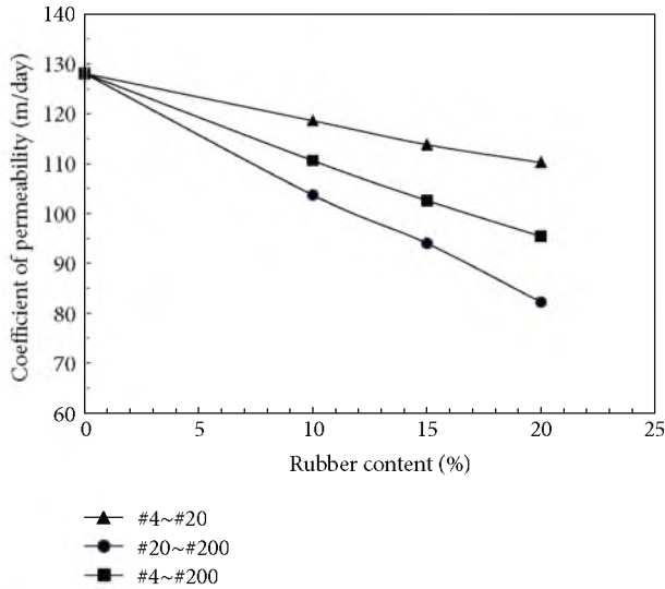
FIGURE 6: Effect of crumb rubber size and content on coefficient of permeability.
