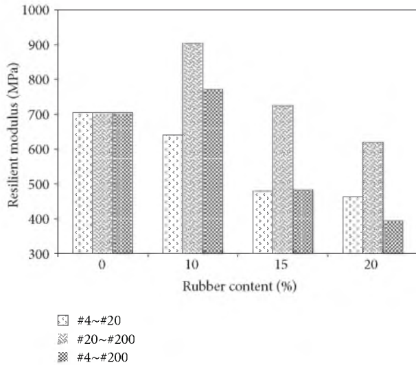
FIGURE 10: Effect of crumb rubber content on resilient modulus.
